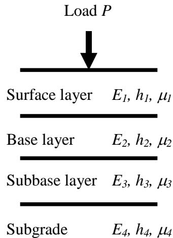
Figure 1: Schematic of four-layer flexible pavement under concentrated load
